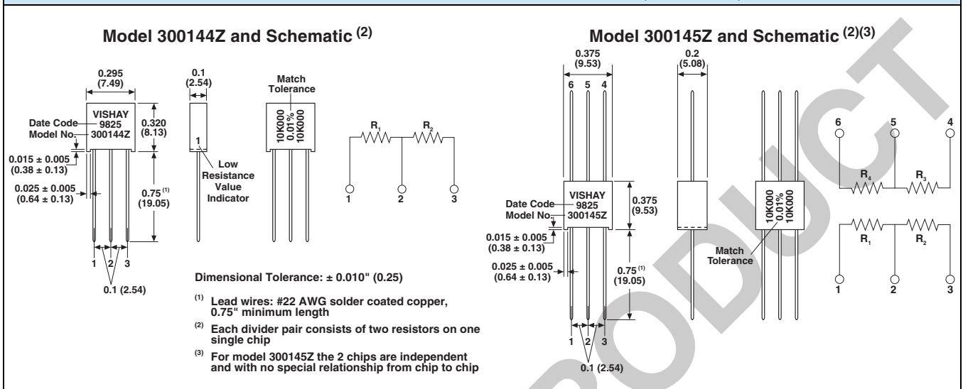
FIGURE 2 - STANDARD PRINTING AND DIMENSIONS in inches (millimeters)
